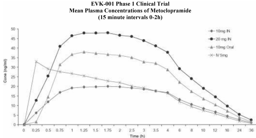
EVK-001 Phase 1 Clinical Trial Mean Plasma Concentrations of Metoclopramide (15 minute intervals 0-2h)
